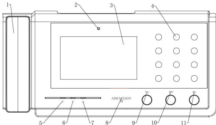
Figure 1-1 Front Panel
